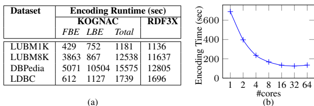
Figure 4: (a) Comparison of KOGNAC vs RDF-3X dictionary encoding times, (b) KOGNAC multi-threading performance analysis on LUBM1K. Experiments on machine M1.
